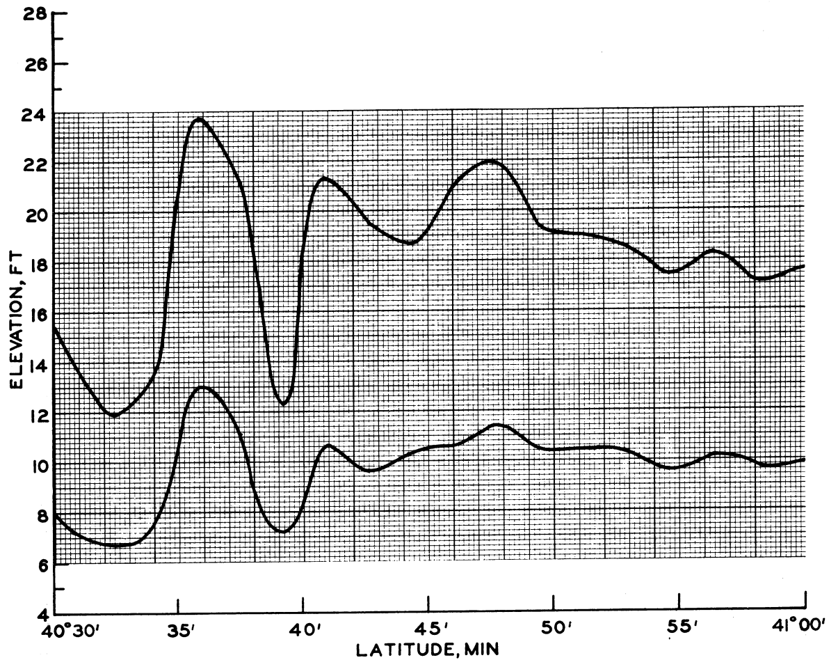
100- AND 500-YEAR ELEVATIONS VS LOCATION LATITUDE 40°30' TO 41°00'
