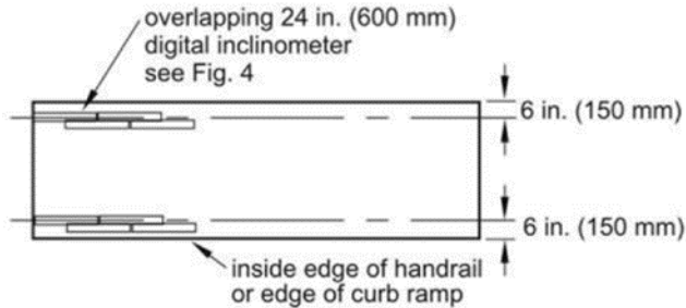
(a) ramps up to and including 5 ft. (1525 mm) wide
