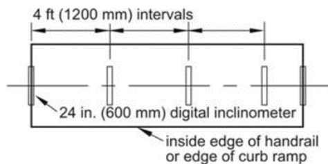
(a) ramps up to and including 5 ft. (1525 mm) wide
