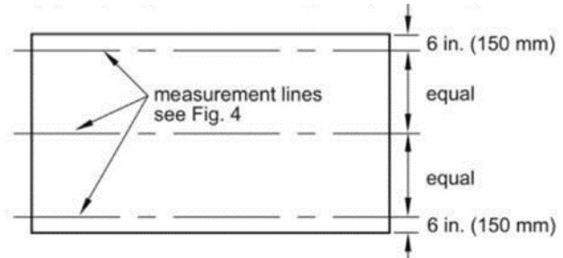
(b) ramps over 5 ft. (1525 mm) wide
