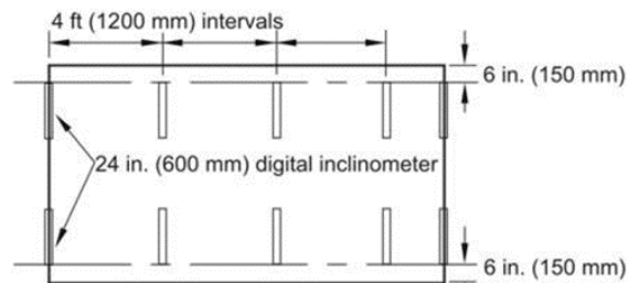
(b) ramps over 5 ft (1525 mm) wide
