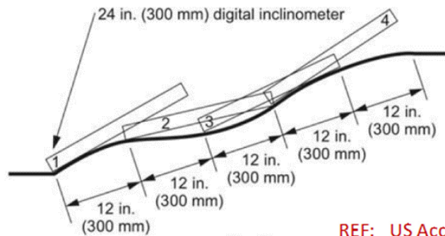
(b) ramps over 5 ft. (1525 mm) wide
