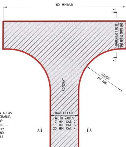
PLAN VIEW ON ROADWAY PARKING PROHIBITED -NOT TO SCALE-
