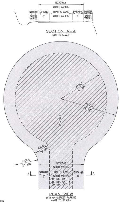
Type 2 On-Street Parking Allowed
