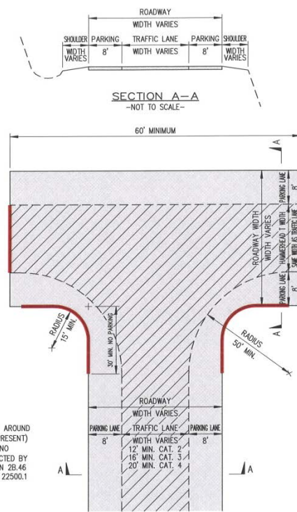
PLAN VIEW ON ROADWAY PARKING ALLOWED -NOT TO SCALE-
