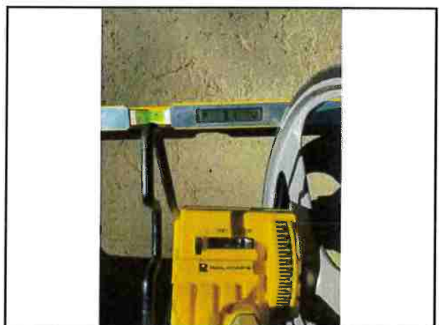
Photo #162 Blue Rock Rd Width 13'7" Slope 3.1 %
