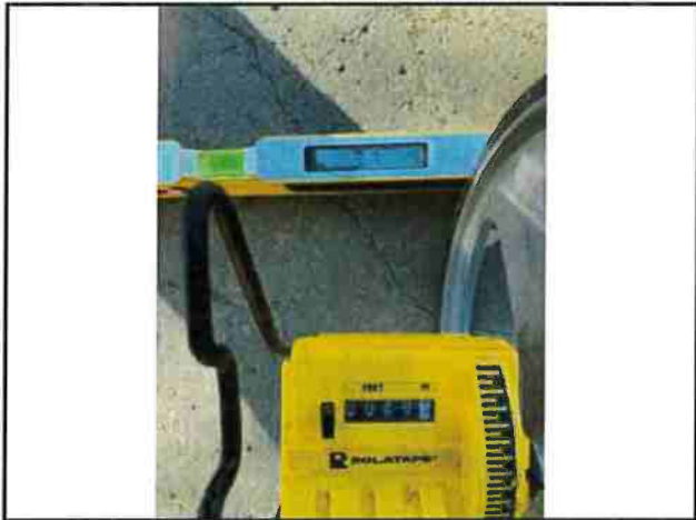
Photo #267 Blue Rock Rd Width 20'1" Slope 3.7%
