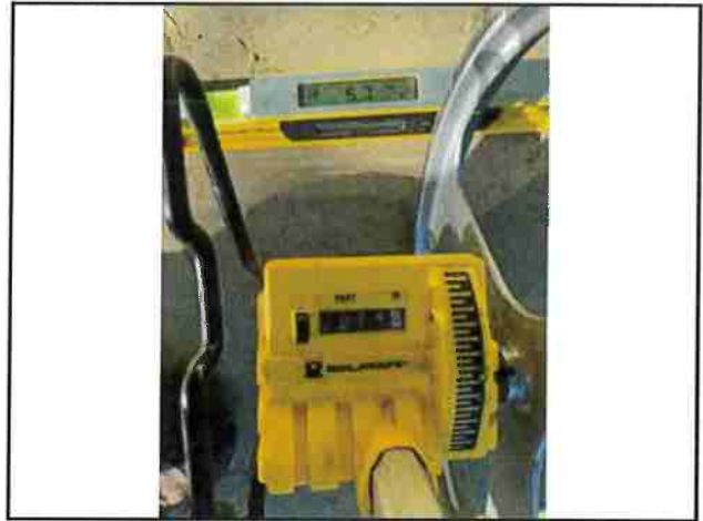
Photo #110 Blue Rock Rd Width 14'0" Slope 5.7%
