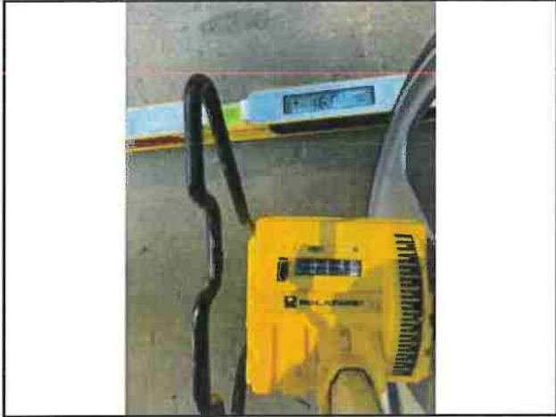
Photo #127 Blue Rock Rd Width 14'10" Slope 16.8%
