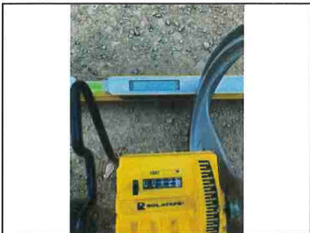
Photo #59 APN #223-034-005 Private Access Rd Width 12'8" Slope 13.3%
