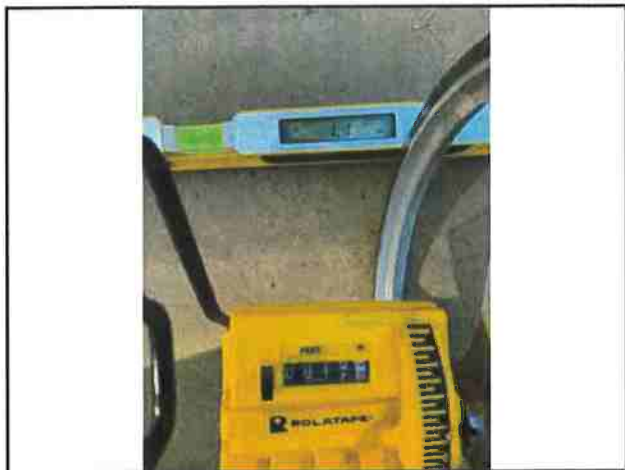
Photo #155 Blue Rock Rd Width 16'0" Slope 1.1 %
