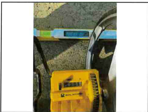
Photo #113 Blue Rock Rd Width 15'2" Slope 11.8%
