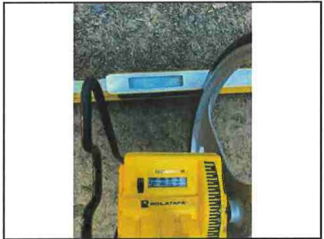
Photo #72 APN #223-034-005 Private Access Rd Width 12'9" Slope 16.2%
