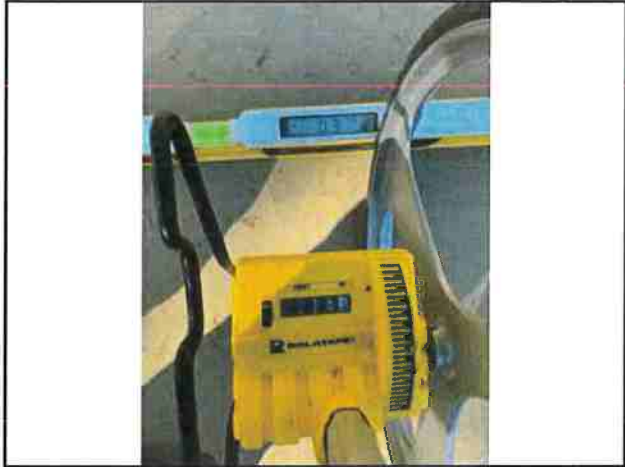
Photo #103 Blue Rock Rd Width 16'8" Slope 0.3%
