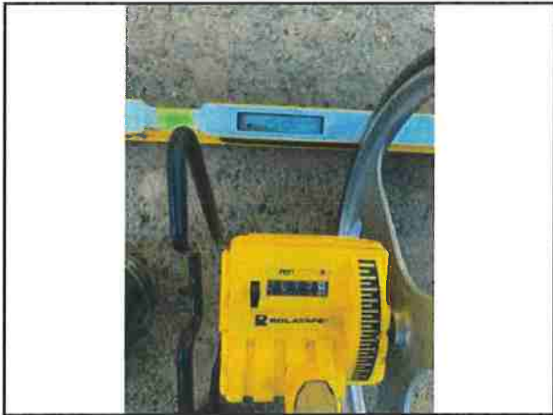
Photo #93 Blue Rock Rd Width 13'2" Slope 16.0%
