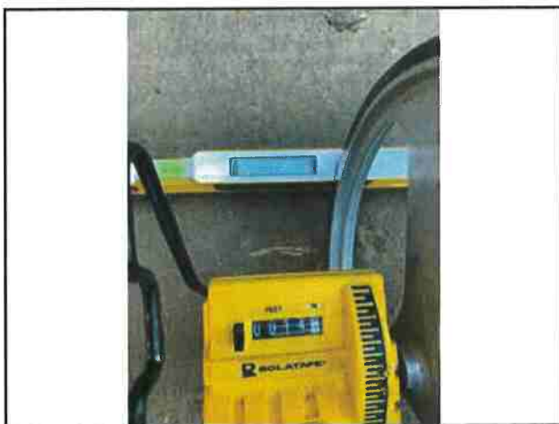
Photo #191 Blue Rock Rd Width 14'1" Slope 11.2%
