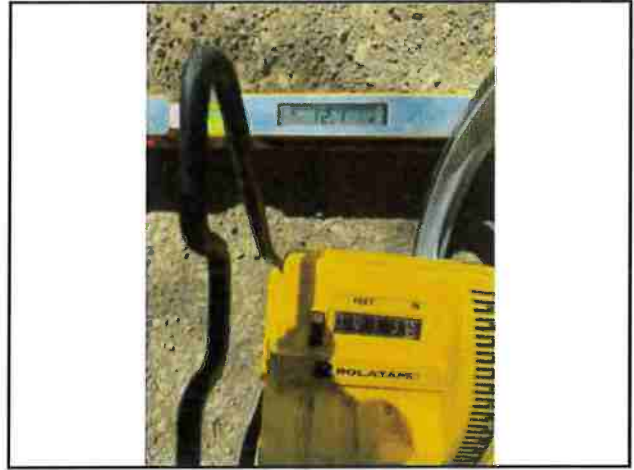
Photo #218 Blue Rock Rd Width 13'9" Slope 12.1%
