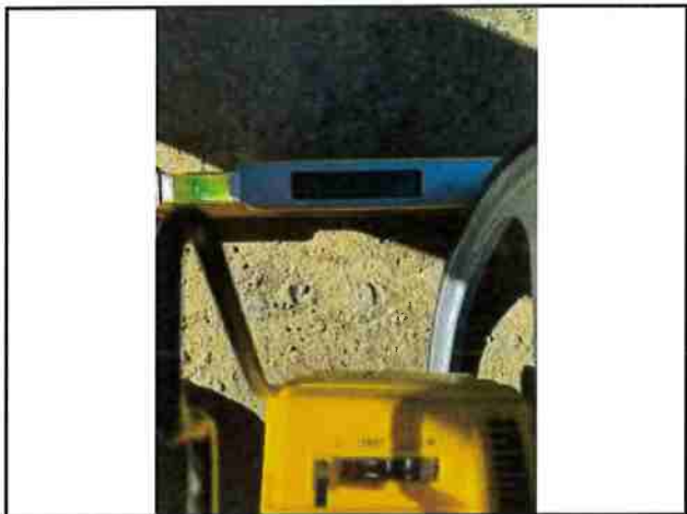
Photo #221 Blue Rock Rd Width 17'1" Slope 7.0%
