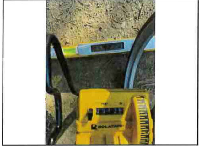
Photo #50 APN #223-034-005 Private Access Rd Width 13'4" Slope 19.2
