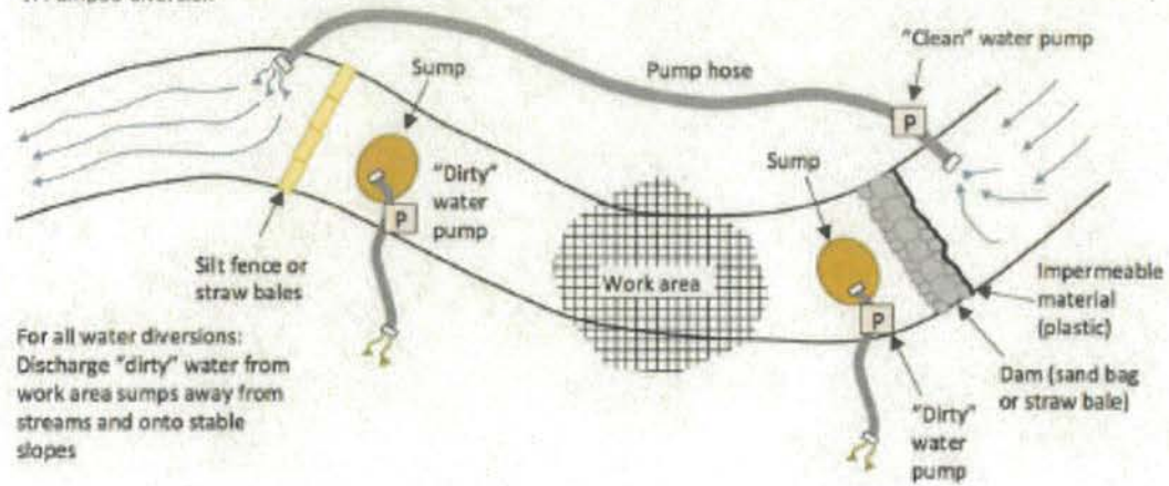
1. Pumped diversion
