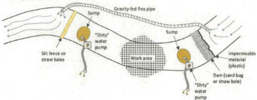
2. Gravity-fed diversion
