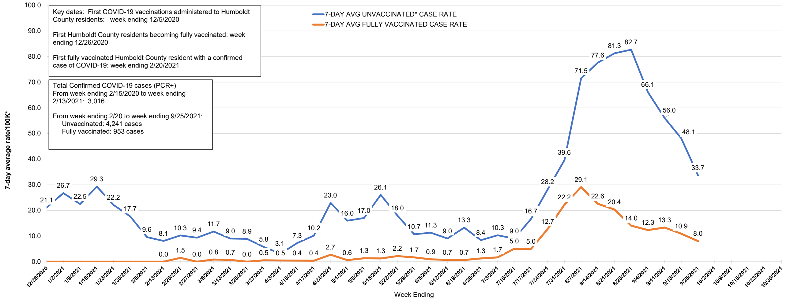
Estimated Humboldt County 7-day average rate per 100,000* newly confirmed COVID-19 cases, vaccinated versus unvaccinated, from week ending 12/26/20 to 9/25/2021 (provisional and subject to change)
