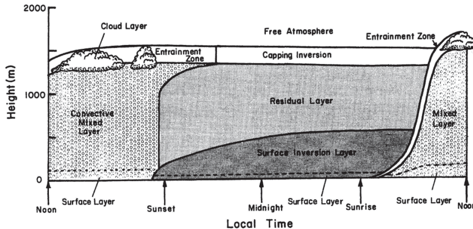
Figure 6: Structure of the convective boundary layer (CBL) according to Stull (1988). The structure of the different parts of the CBL coincides perfectly with the distribution of insect density during the day found by Contreras and Frasier (2008) shown in the following Figure 7.
