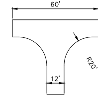
SRA HAMMERHEAD TURN AROUND DETAIL
