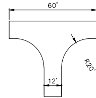
SRA HAMMERHEAD TURN AROUND DETAIL
