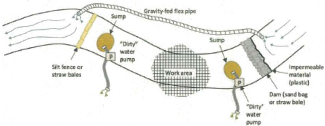
2. Gravity-fed diversion
