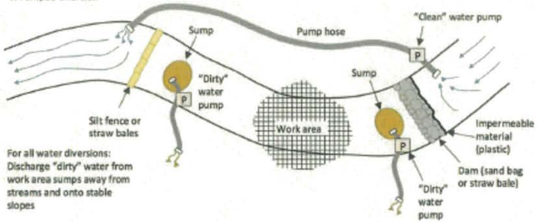
1. Pumped diversion
