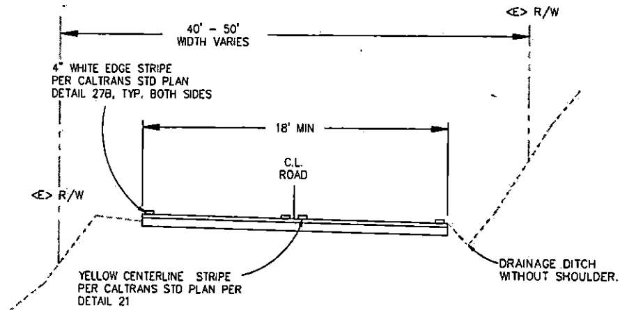
TYPICAL ROAD SECTION 18' MINIMUM N.T.S.
