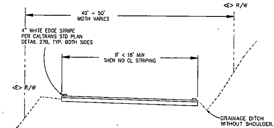
TYPICAL ROAD SECTION LESS THAN 18' WIDTH N.T.S.
