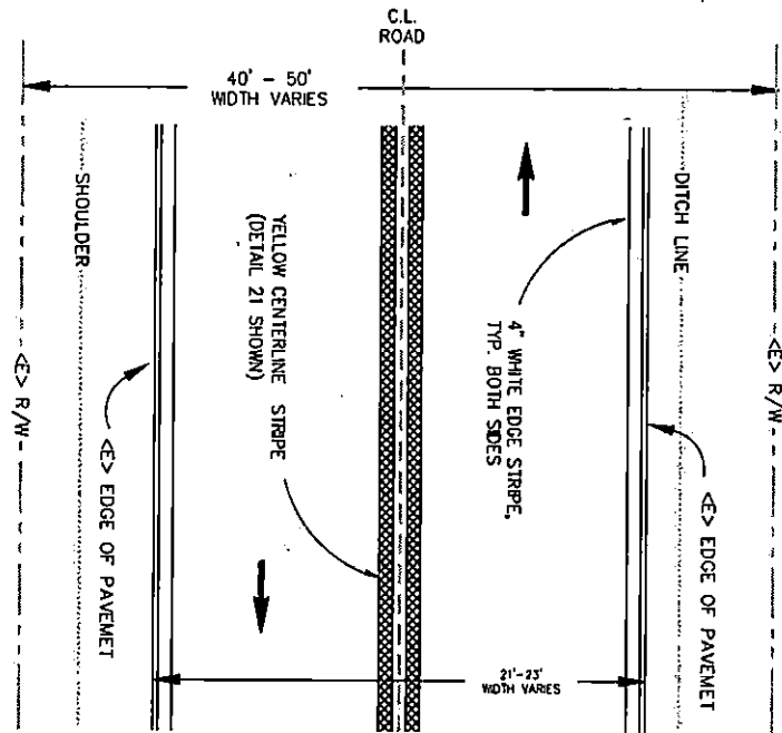
TYPICAL PLAN VIEW N.T.S.
