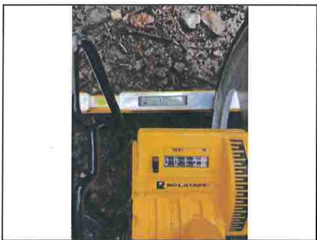
Photo #118 Kings Peak Rd Slope 1.8% Width 15'11"
