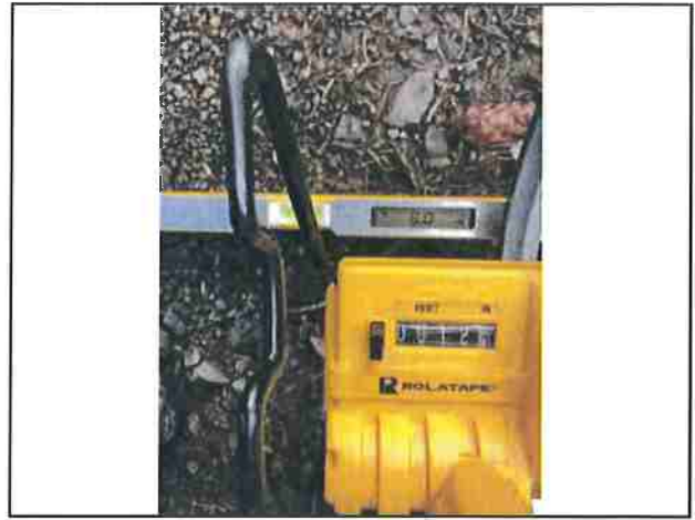
Photo #158 Kings Peak Rd Slope 8.0% Width 12'3"
