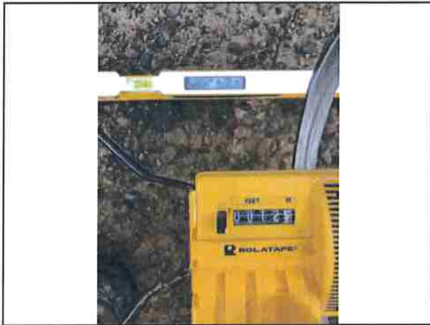
Photo #75 Kings ZPeak Rd Slope 2.6% Width 12'4"
