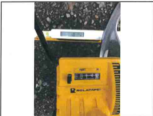
Photo #143 Kings Peak Rd Slope 11.0% Width 14'10"
