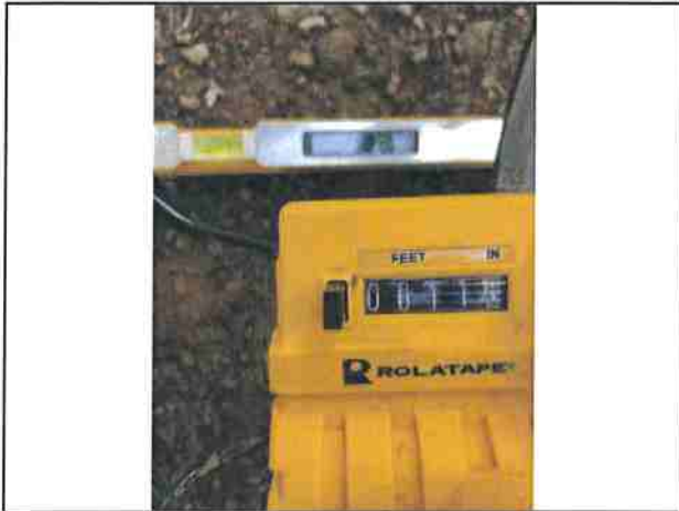
Photo #45 Kings Peak Rd Slope 10.8% Width 11'8"
