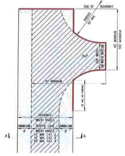
PLAN VIEW ON ROADWAY PARKING ALLOWED -NOT TO SCALE-
