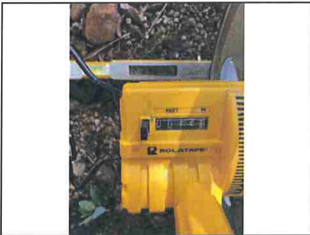
Photo #5 Private Access Rd Slope 23.6% Width 12'1"
