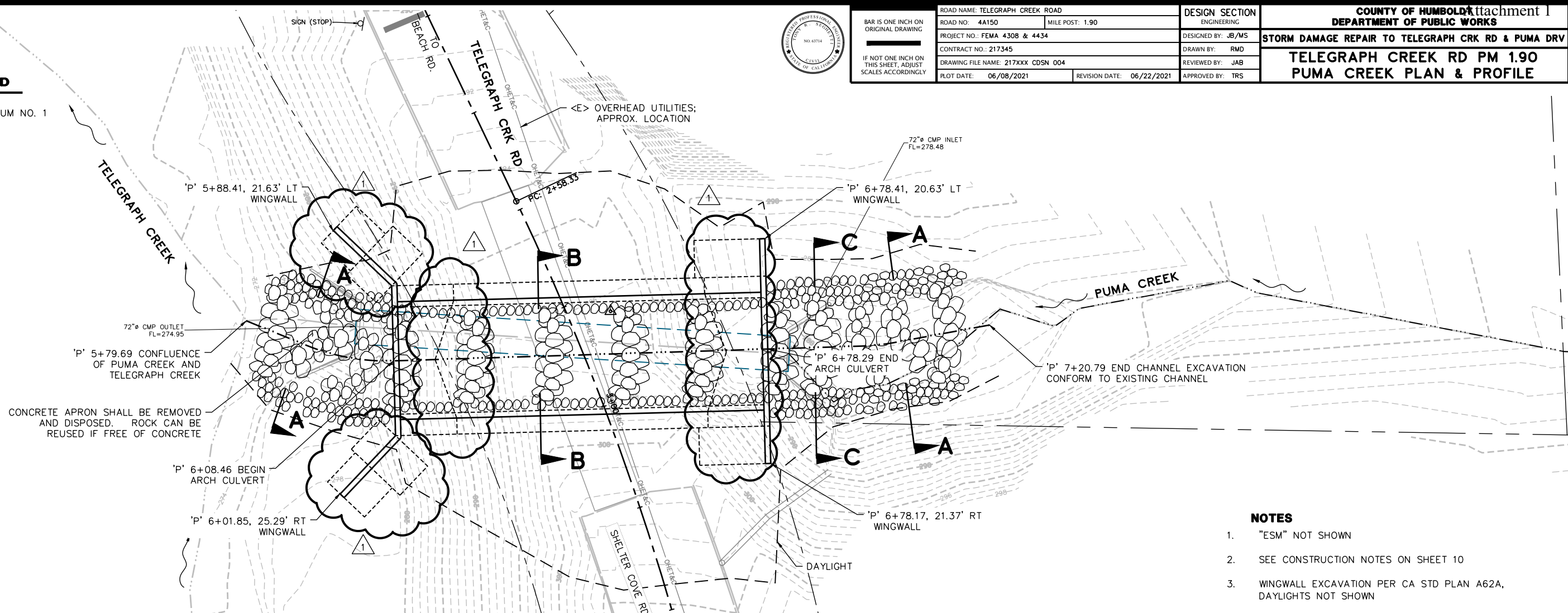
PLAN VIEW
