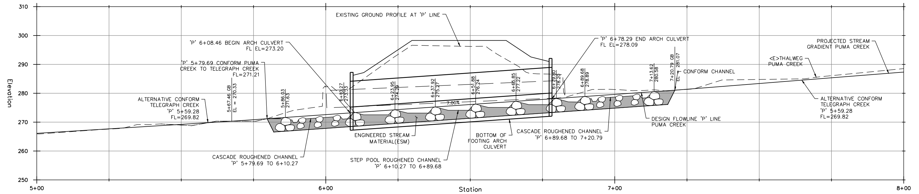
PROFILE VIEW
