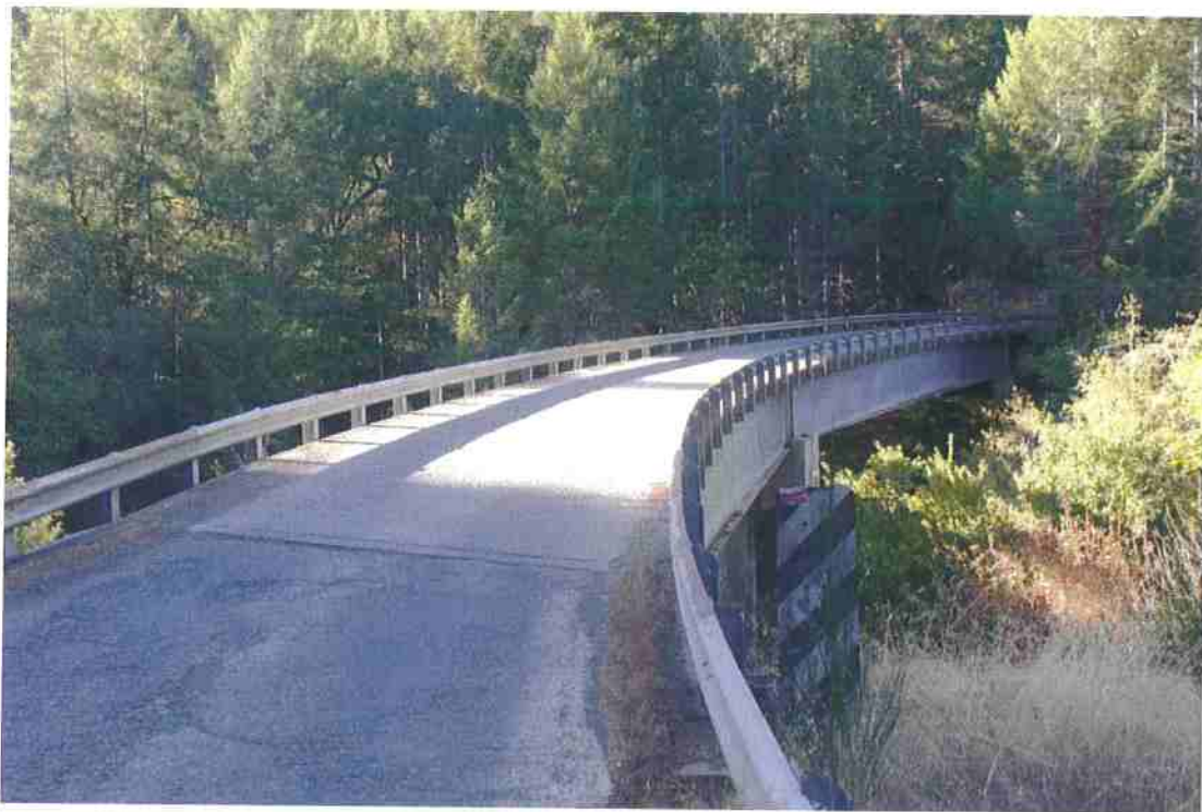
Photo 38. Mile 3.3: 16-ft wide bridge, no shoulders. Recommend removing vegetation on west extent of bridge to improve visibility.
