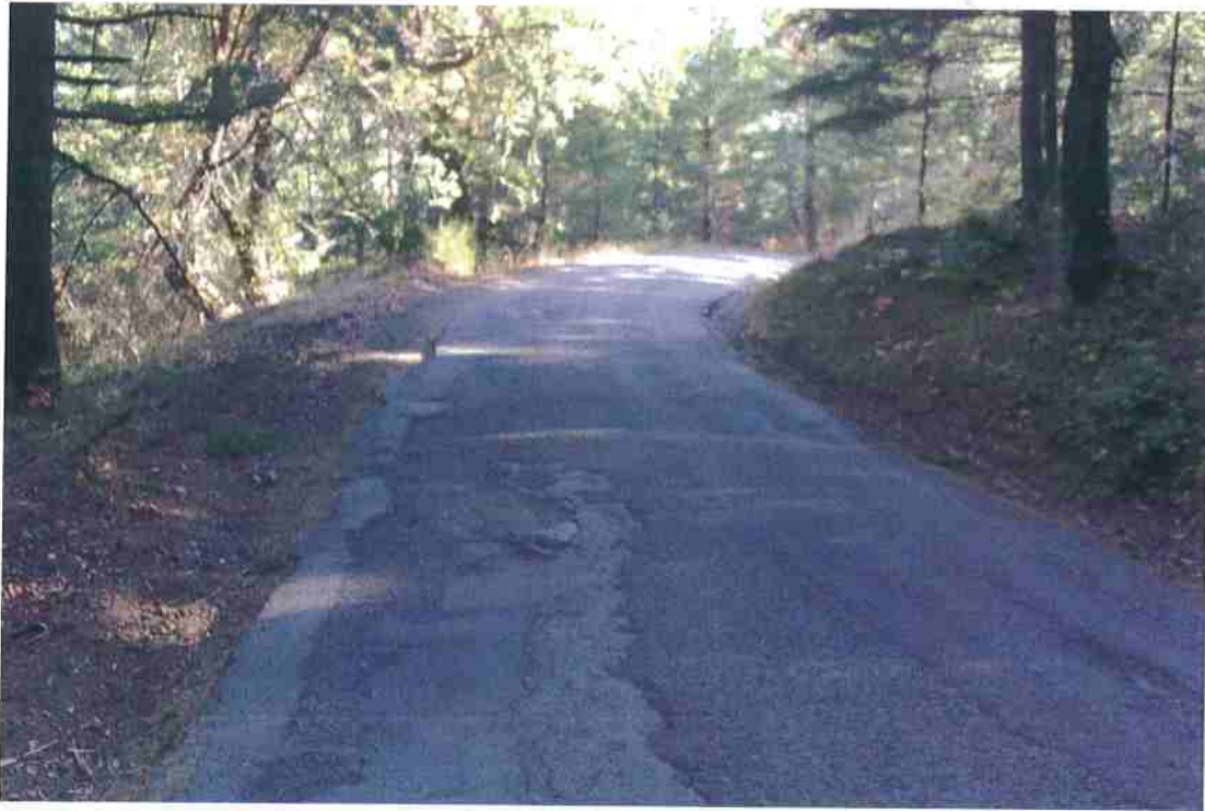
Photo 46. Mile 3.9: 15-ft road width with 2-ft shoulders. Broken pavement edges make segment more treacherous.
