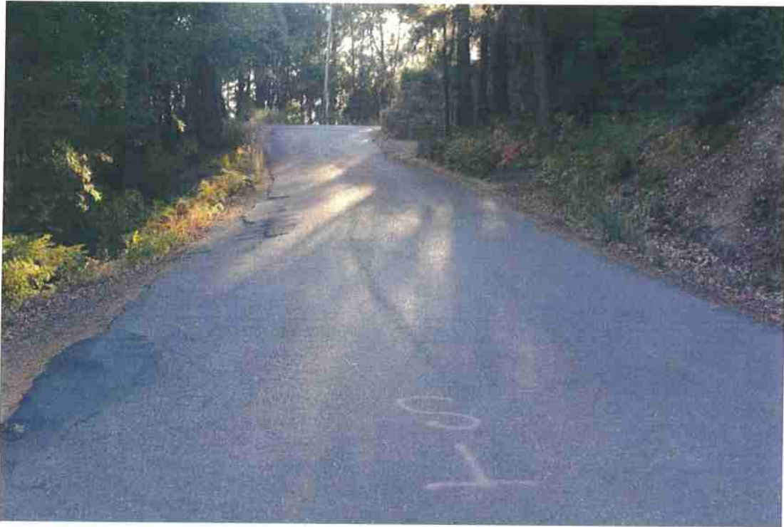
Photo 19. Mile 1.8: 20-ft road width with 2-ft shoulders.
