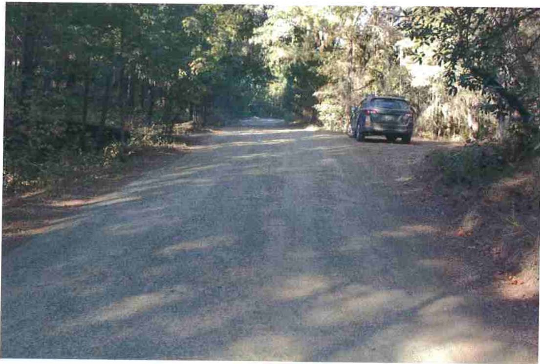
Photo 6. Mile 0.4: 18-ft road width with 1-ft shoulder.
