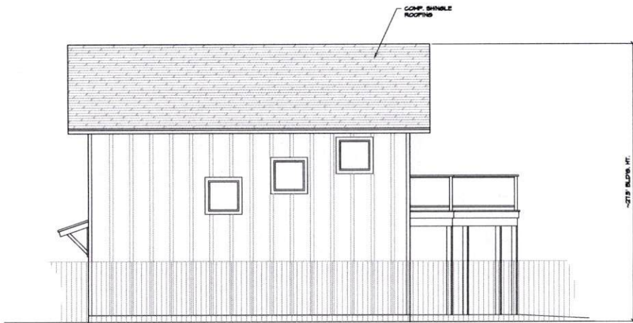
NORTH ELEVATION 1/4"=1'-0"
