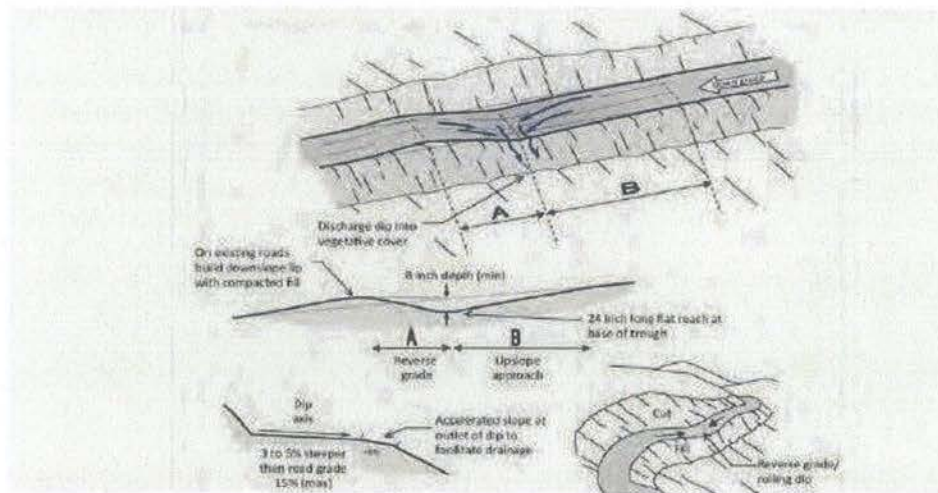
FIGURE 34. A classic Type I rolling dip, where the excavated up-road approach (B) to the rolling dip is several percent steeper than the approaching road and extends for 80 to 80 feet to the dip axis. The lower side of the structure reverses grade (A) over approximately 15 feet or more, and then falls down to rejoin the original road grade. The dip must be deep enough that it is not obliterated by normal grading, but not so deep that it is difficult to negotiate or a hazard to normal traffic. The outward cross-slope of the dip axis should be 3% to 5% greater than the up-road grade (B) so it will drain properly. The dip axis should be out-sloped sufficiently to be self-cleaning, without triggering excessive downcutting or sediment deposition in the dip axis (Modified from: Best, 2013).
