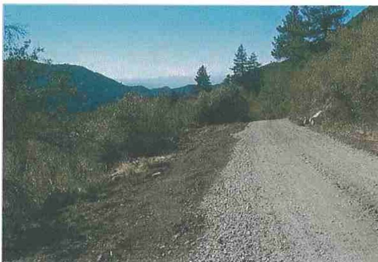
Figure 1. Low-volume road that has been newly gravelled and out-sloped, San Bernardino County. Photo: Richard Harris.
