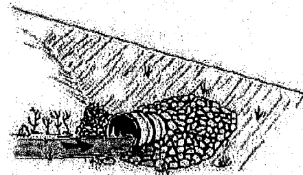
FIGURE 107B. Riprap armor at culvert inlet (Keller and Spector, 2003).
