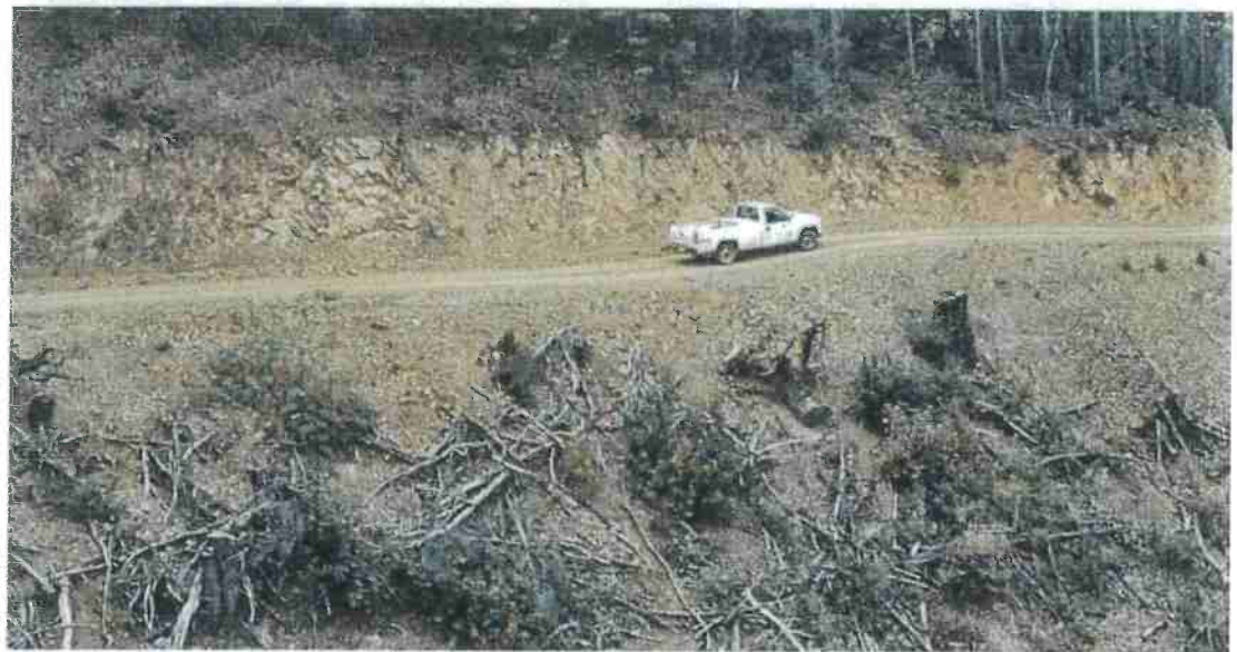
FIGURE 33B. This side view of an outsloped road shows that the rolling dip does not have to be deep or abrupt to reverse road grade and effectively drain the road surface. This outsloped forest road has rolling dips that allow all traffic types to travel the route without changing speed.
