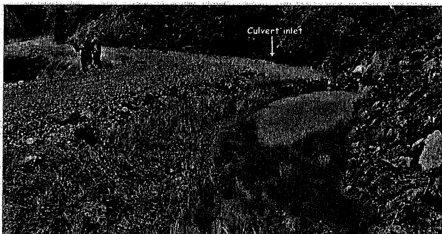
FIGURE 238. Traffic and surface runoff from gravelled roads often produces surface erosion, turbid runoff and fine sediment transport that can be delivered to streams. Where ditches can't be eliminated, sediment traps and roadside settling basins can be installed to capture and remove most of the eroded sediment. This settling basin has been constructed along the inside ditch just before a stream crossing culvert inlet (see arrow). Eroded sediment from the road and ditch are deposited in the basin before flow is released to the stream. Fine sediments have filled about 1/3 of this basin and vegetation is now growing. Sediment basins require periodic maintenance to maintain their storage capacity.
