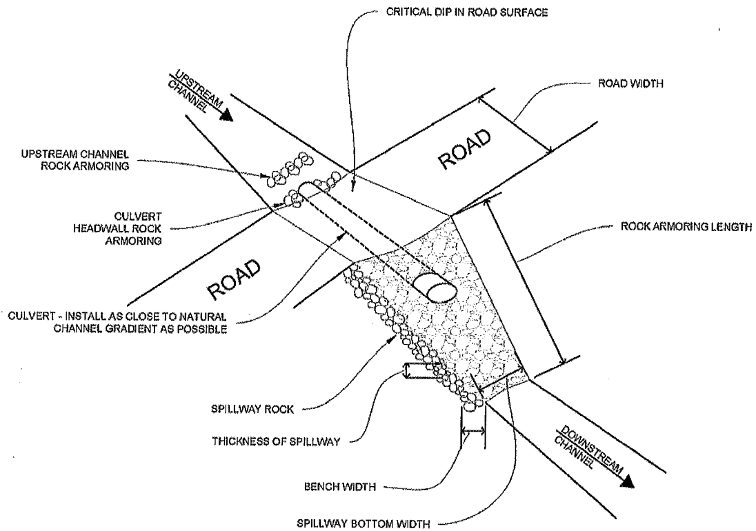
Figure 4. Culvert installation schematic.
