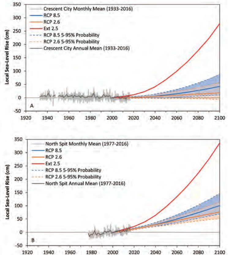
Local sea level projections at Crescent City (A) and Humboldt Bay "North Spit" (B) for high-emissions (RCP 8.5) and low-emissions (RCP 2.6) scenarios, based on data from Kopp et al. (2014), and an extreme (Ext 2.5) sea-level rise scenario from Sweet et al. (2017). The 5th and 95th percentile probabilities are the shaded areas bounded by dashed lines (Source: Anderson 2018).
