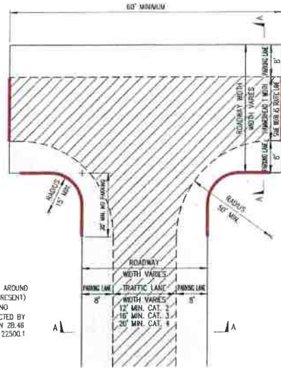
PLAN VIEW ON ROADWAY PARKING ALLOWED -NOT TO SCALE-
