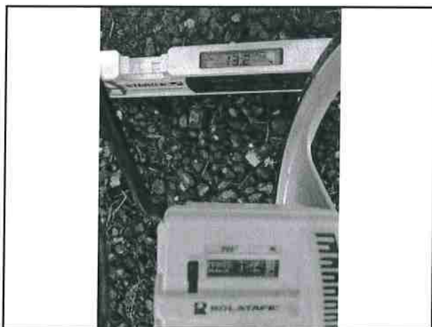
Photo #29 Private Driveway on APN 208-341-021 Slope 13.2% Width 12'7"
