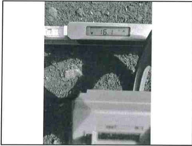
Photo #13 Cob Rd Slope 16.1% Width 12'7"
