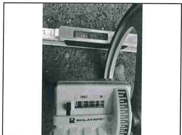
Photo #18 Cobb Rd Slope 15.1% Width 13'2"
