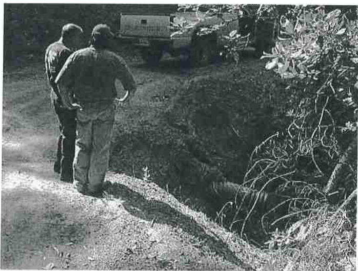
Figure 14. This fill slope erosion was caused by a plugged cross-drain inlet that diverted ditch flow over the road surface. Photo: Angela Wilson, Central Valley Regional Water Quality Control Board.
