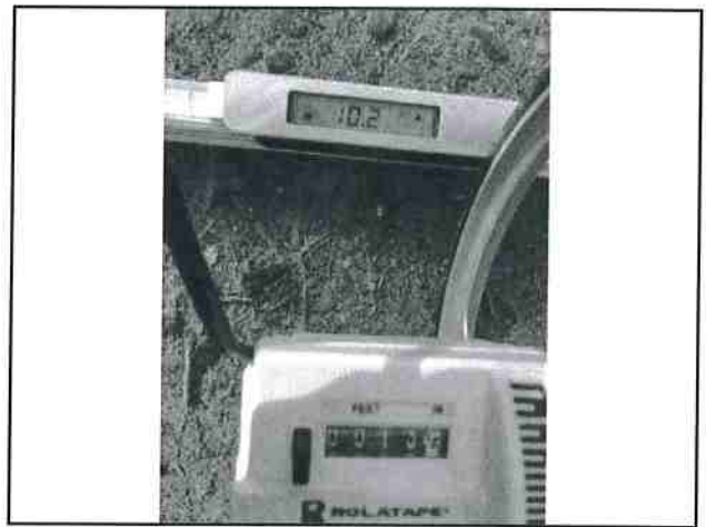
Photo # 32 Cobb Rd Slope 10.2% Width 13'5"
