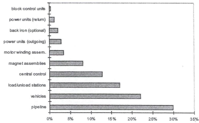
Figure 10 Line Length = 2.7 km (1.72 mi.) Component Cost Histogram at the Optimum Operating Point of 26" Pipeline, 20 mph
