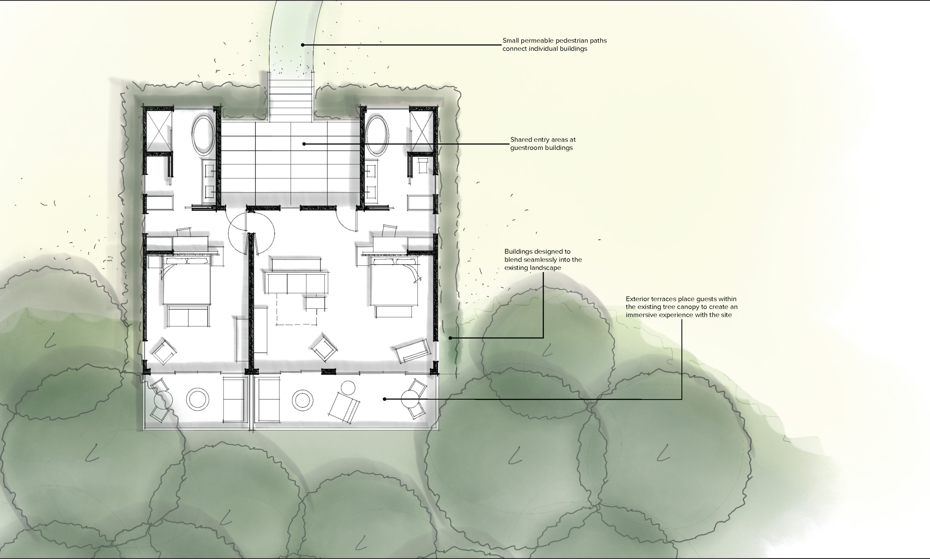
Typical Guestroom Building - 1/8" = 1'-0"
