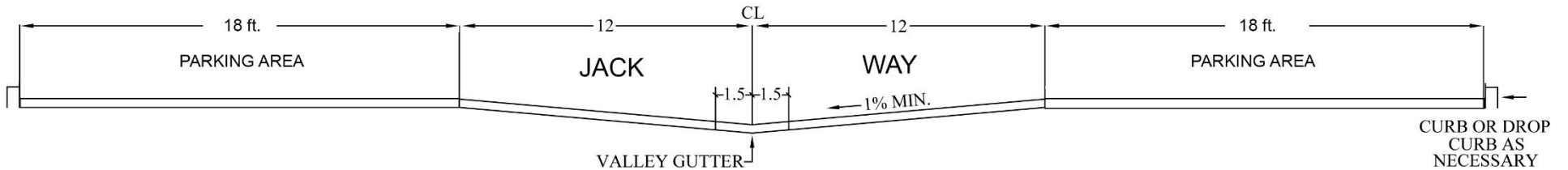
PROPOSED CROSS SECTION FOR 24 FT. WIDE RIGHT OF WAY
