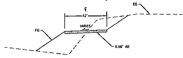
TYPICAL DISPOSAL SITE SECTION SCALE: 1"=5'
