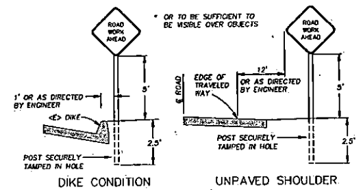
RURAL CONSTRUCTION AREA SIGN - NOT TO SCALE -
