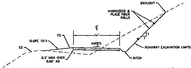
TYPICAL ROADWAY SECTION SCALE: 1"=5'
