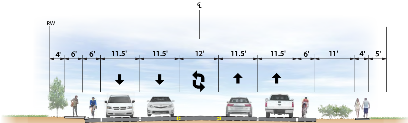
CENTRAL AVENUE - EXISTING School Road to Railroad Drive
