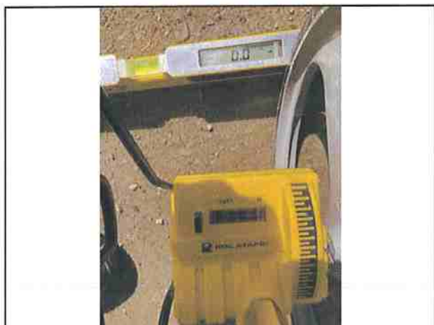
Photo #185 Showers Pass Rd Slope 0.0% Width 14'1"
