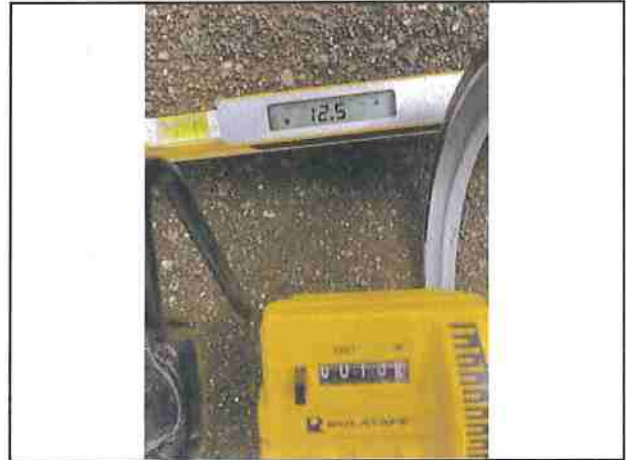
Photo #230 Showers Pass Rd Slope 12.5% Width 13'3"
