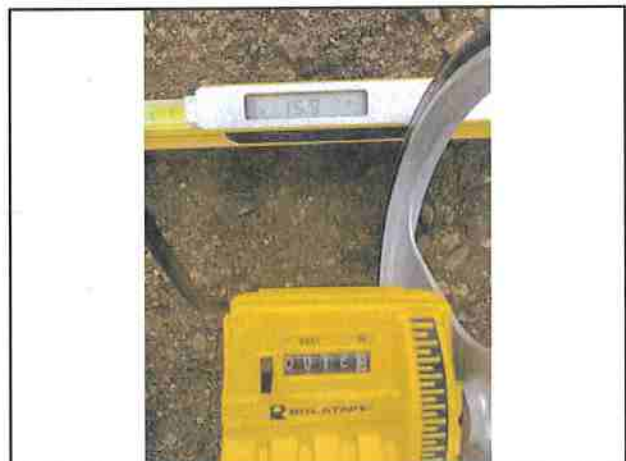
Photo #78 Gorden Rd Slope 15.9% Width 12'10"
