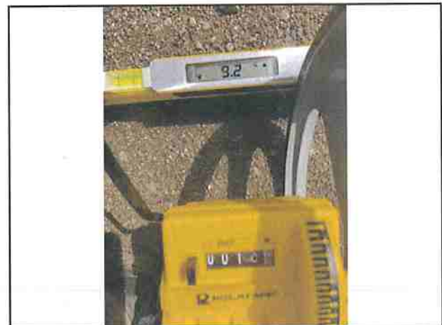
Photo #246 Showers Pass Rd Slope 9.2% Width 13'2"
