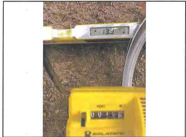
Photo #22 Private Access Rd APN APN 317-023-010 Slope 13.3% Width 10'2"
