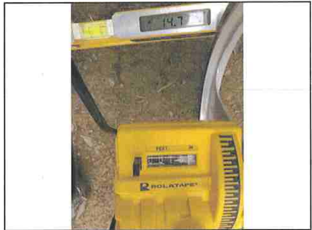
Photo 338 Showers Pass Rd Slope 14.7% Width 15'11"
