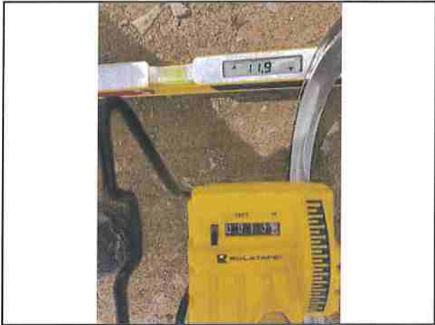
Photo #353 Showersw Pass Rd Slope 11.9% Width 13'5"
