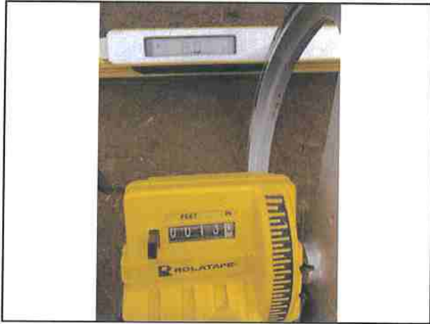
Photo #7 Private Access Rd APN APN 317-023-010 Slope 8.0% Width 13'0"
