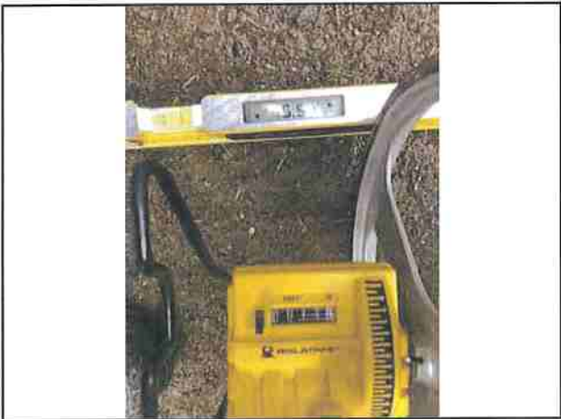
Photo #63 Gorden Rd Slope 15.5% Width 11'0"
