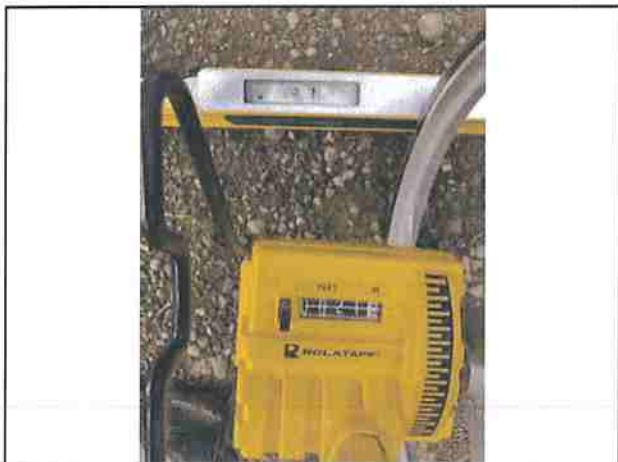
Photo #309 Showers Pass Rd Slope 13.7% Width 21'6"
