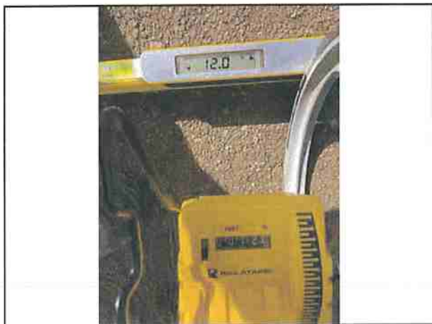
Photo #215 Showers Pass Rd Slope 12.0% Width 12'6"
