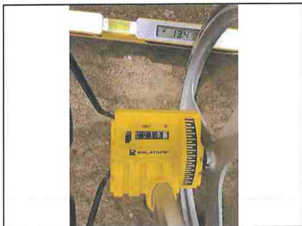
Photo #339 Showers Pass Rd Slope 15.7% Width 15'7"
