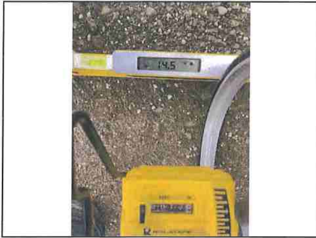
Photo #235 Showers Pass Rd Slope 14.5% Width 13'8"
