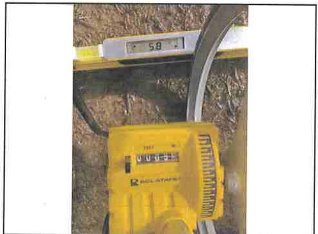
Photo #12 Private Access Rd APN APN 317-023-010 Slope 5.8% Width 9'10"
