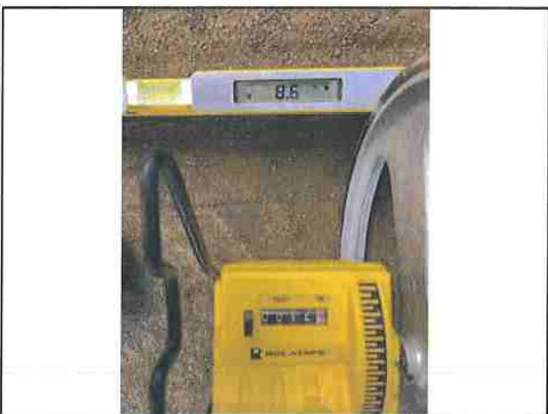
Photo #191 Showers Pass Rd Slope 8.6% Width 12'10"
