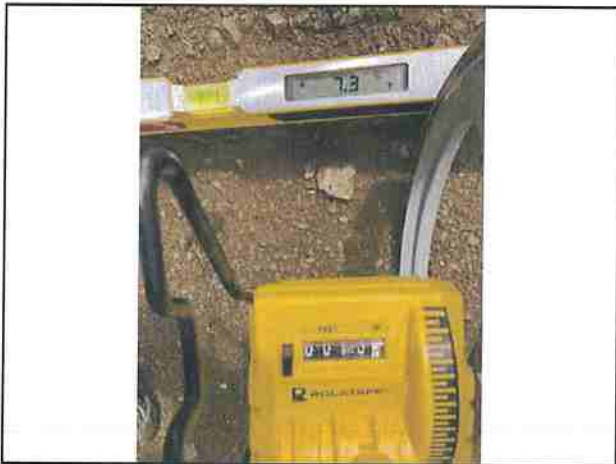
Photo #363 Showers Pass Rd Slope 7.3% Width 13'8"
