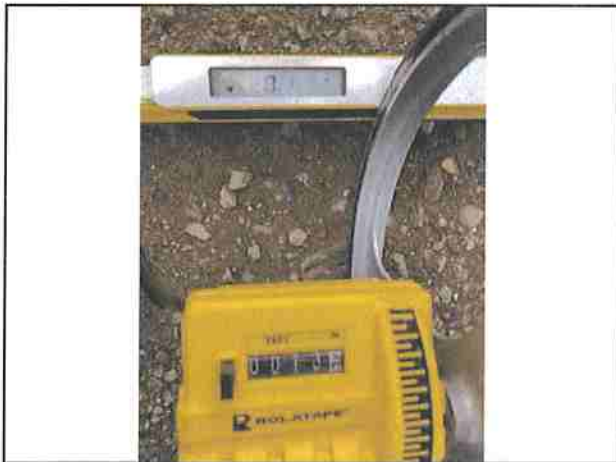
Photo #261 Showers Pass Rd Slope 9.4% Width 15'3"
