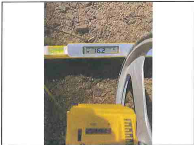
Photo #181 Showers Pass Rd Slope 16.2% Width 13'9"
