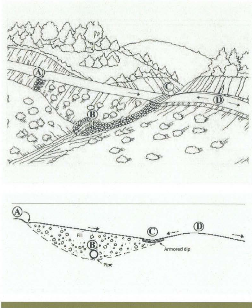
FIGURE 84. Critical dips or dipped crossing fills should be centered near a stream crossing's down-road hingeline, not over the centerline of the crossing where overtopping could cause washout or severe erosion of the fill. If the stream crossing culvert (B) plugs, water will pond behind the fill until reaching the critical dip or low point in the crossing (C) and flowing back down into the natural stream channel. The down-road ditch must be plugged to prevent streamflow from diverting down the ditch line. For extra protection in this sketch, riprap armor has been placed at the critical dip outfall and extending downslope to the stream channel. This is only required or suggested on stream crossings where the culvert is highly likely to plug and the crossing fill overtopped. The dip at the hinge line is usually sufficient to limit erosional damage during an overtopping event. Road surface and ditch runoff is disconnected from the stream crossing by installing a rolling dip and ditch relief culvert just up-road from the crossing (A) (Keller and Sherar, 2003).
