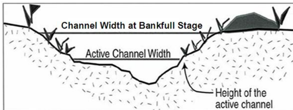
Figure 4: Depiction of channel width at Bankfull stage compared to Active Channel width (modified from California Department of Fish and Game's (CDFG) Salmonid Stream Habitat Restoration Manual, Taylor and Love, 2003).
