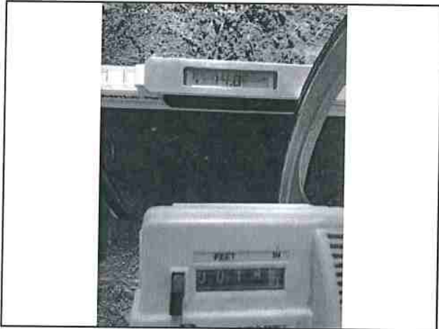
Photo #9 APN 208-241-019 Private Access Rd Width 14'7" Slope 14.0%
