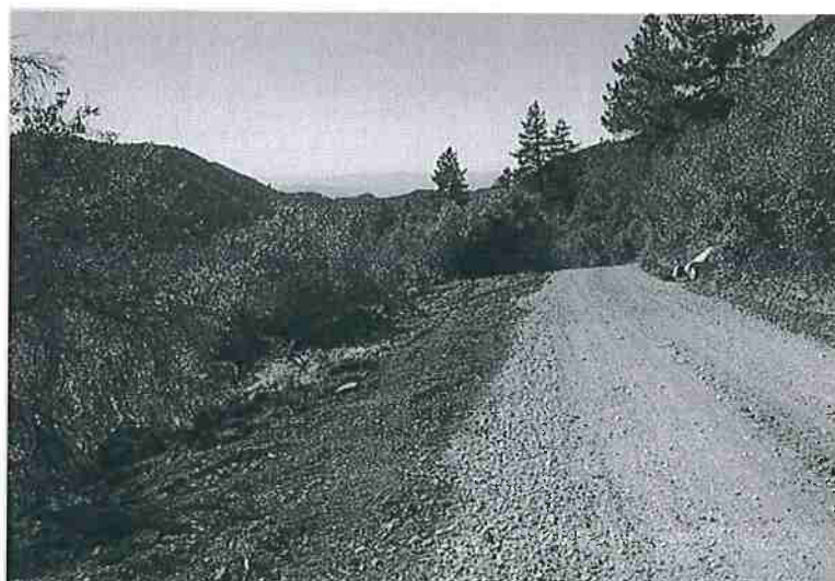
Figure 1. Low-volume road that has been newly graveled and out-sloped, San Bernardino County. Photo: Richard Harris.
