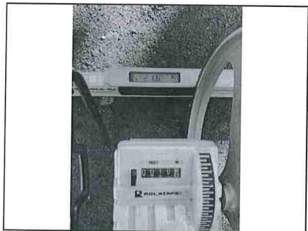
Photo # 6 APN 208-241-019 Private Access Rd Width 10'2" Slope 21.6%
