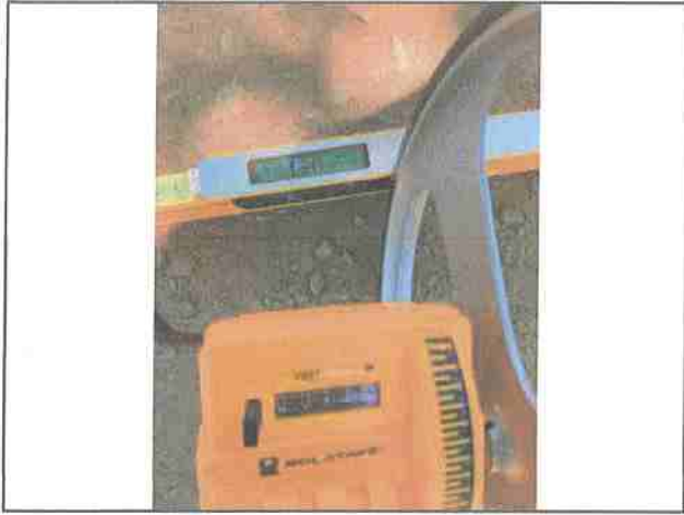
Photo #193 Thomas Rd Slope 15.0% Width 17'0"
