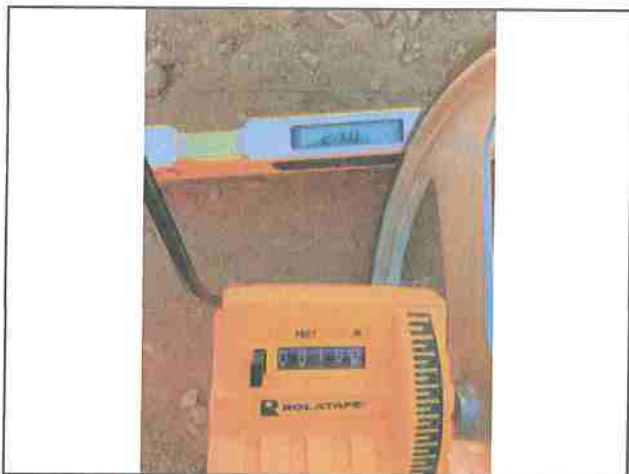
Photo #35 Private Access Rd APN 221-071-020 Slope 21.0% Width 10'5"
