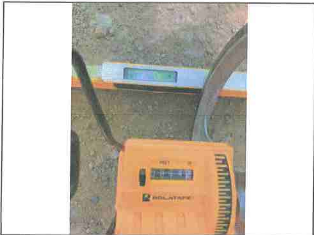
Photo #309 Thomas Rd Slope 15.7% Width 14'9"
