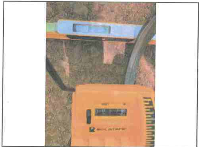
Photo #232 Thomas Rd Slope 12.1% Width 17'8"
