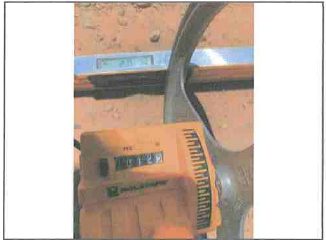
Photo #148 Salmon Creek Rd Slope 2.0% Width 12'2"
