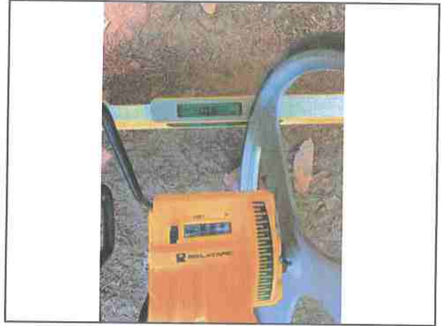
Photo #116 Private Access Rd APN 221-071-020 SAlope 10.6% Width 13'9"
