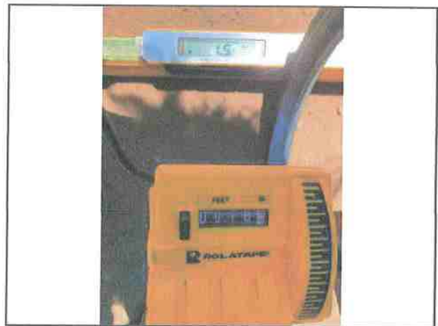
Photo #222 Thomas Rd Slope 1.5% Width 18'4"
