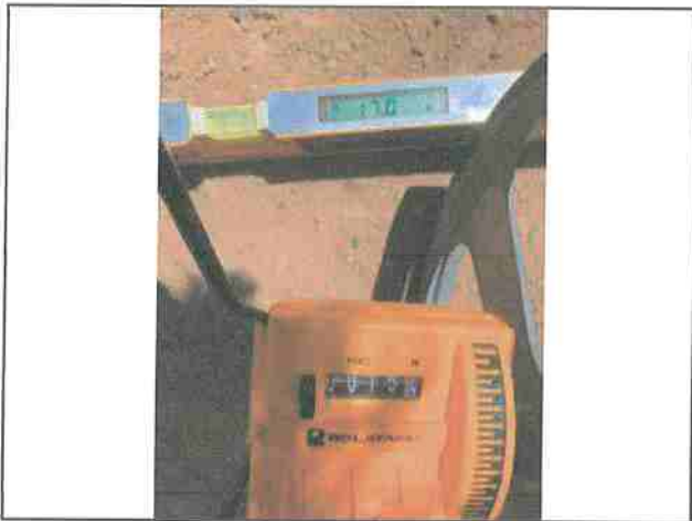
Photo #189 Thomas Rd Slope 17.4% Width 15'4"
