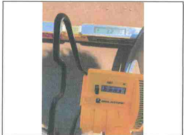
Photo #154 Salmon Creek Rd Slope 3.2% Width 13'2"
