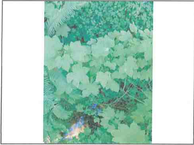
Photo #241 Thomas Rd Looking @ Partially Clogged Culvert Inlet
