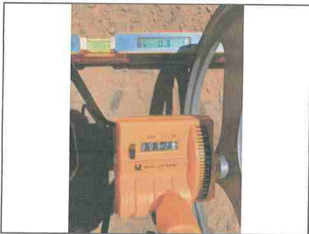
Photo #167 Thomas Rd Slope 0.3% Width 17'2"
