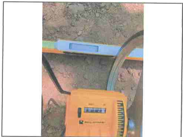
Photo #54 Private Access Rd APN 221-071-020 Slope 17.7% Width 13'7"
