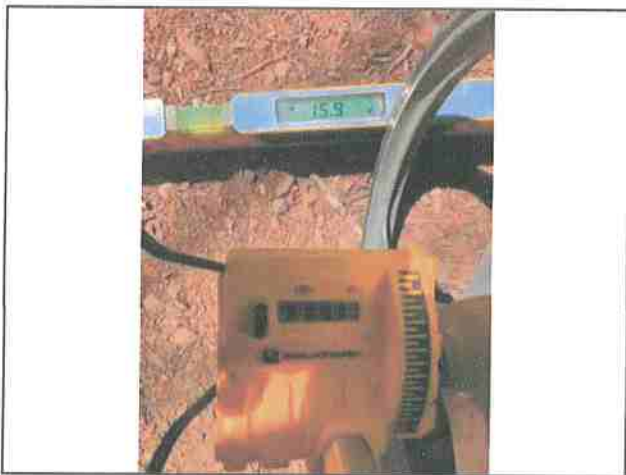
Photo #23 Private Access Rd APN 221-071-020 Slope 15.9% Width 10'10"
