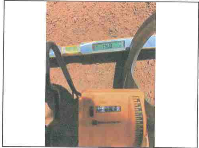
Photo #140 Salmon Creek Rd Slope 14.8% Width 12'2"
