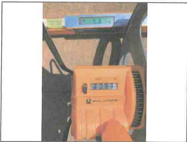
Photo #203 Thomas Rd Slope 5.3% Width 15'10"
