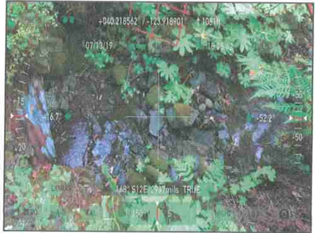
Photo #74 Private Access Rd APN 221-071-020 Looking @ 30" Culvert Size Inlet
