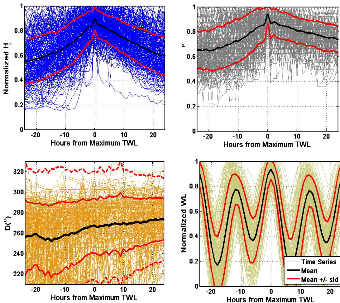
Figure 7. Time series of environmental wave (height ( H_s ), period ( T_p ), and direction ( D^{\circ} ) and water level water level (WL) conditions associated with the 191 extreme storm events selected to represent the synthetic storm for the XBeach storm scenario analysis. Note that wave height, period, and water level were normalized.
