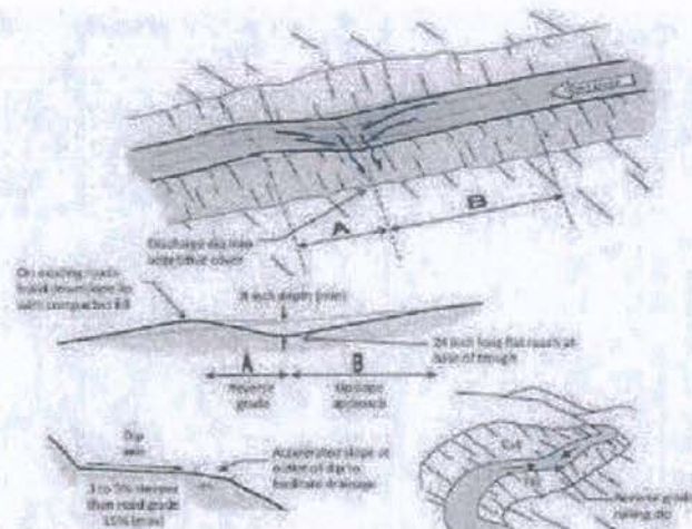
FIGURE 34. A classic Type I rolling dip, where the excavated up-road approach (B) to the rolling dip is several percent steeper than the approaching road and extends for 60 to 90 feet to the dip axis. The lower side of the structure reverses grade (A) over approximately 15 feet or more, and then falls down to regain the original road grade. The dip must be deep enough that it is not obliterated by normal grading, but not so deep that it is difficult to negotiate or a hazard to normal traffic. The outward cross-slope of the dip axis should be 3% to 5% greater than the up-road grade (B) so it will drain properly. The dip axis should be out-sloped sufficiently to be self-cleaning, without requiring excessive downcutting or sediment deposition in the dip axis (Modified from: Best, 2013).
