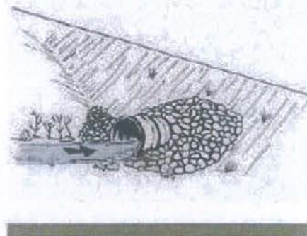
FIGURE 107B. Riprap armor at culvert inlet (Keller and Sherat, 2003).
