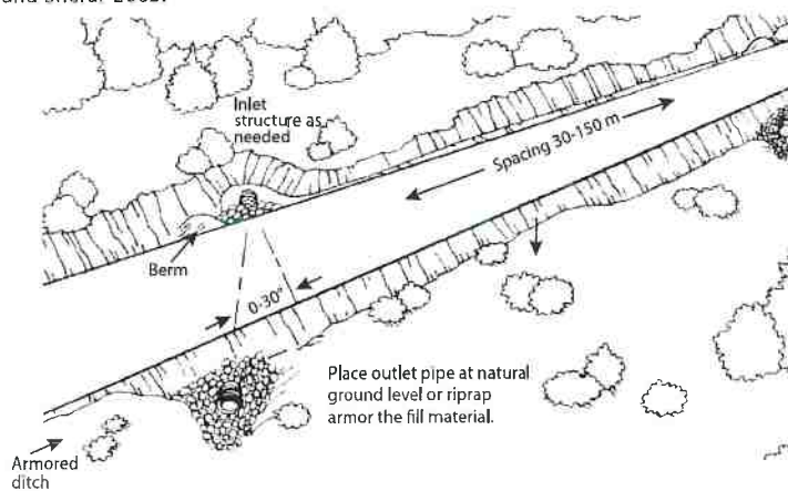
Figure 13B. Installation of ditch relief culverts on an in-sloped road section. Source: Keller and Sherar 2003.
